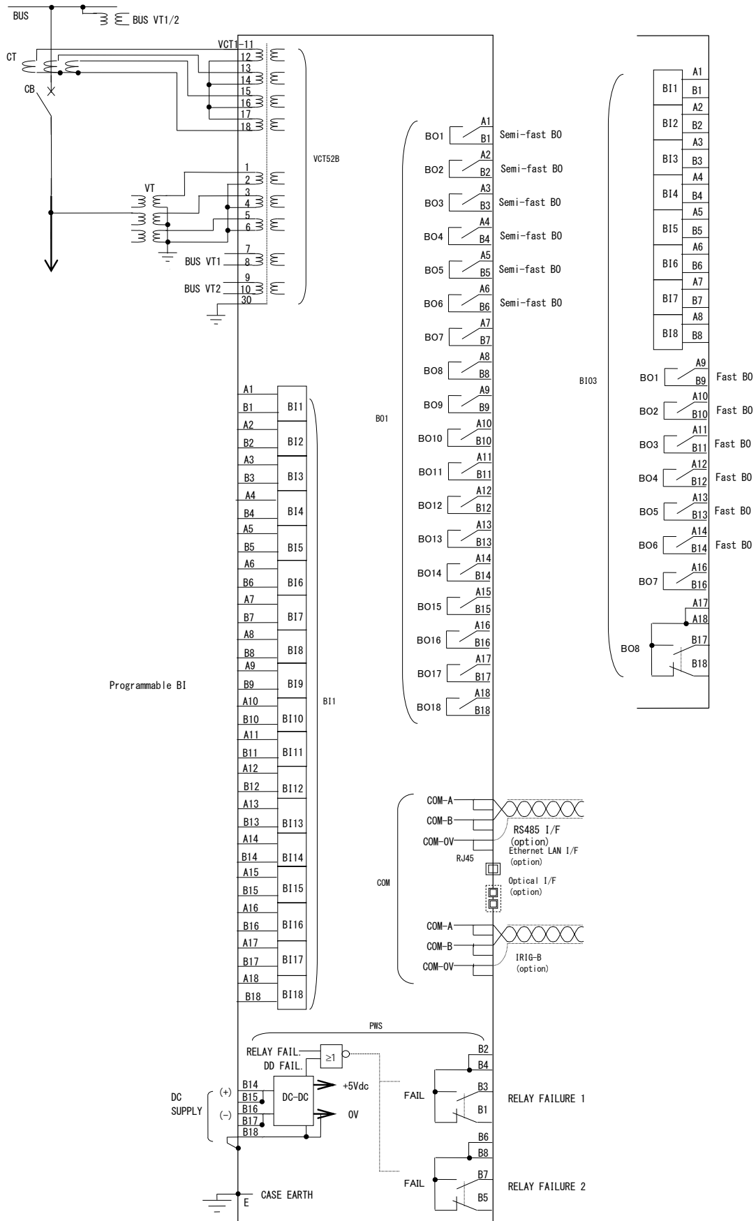
Figure 15 – Typical external connection diagram – ring terminal type (VCT: No.52, IO: B11, BO1 and B103)
