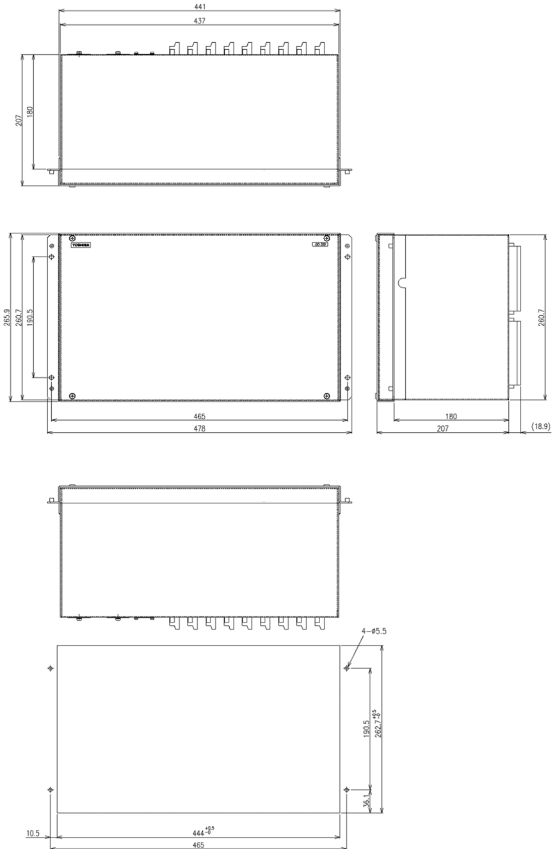
Figure 17 – Dimension and Panel Cut-out – 1/1 x 19” case size
