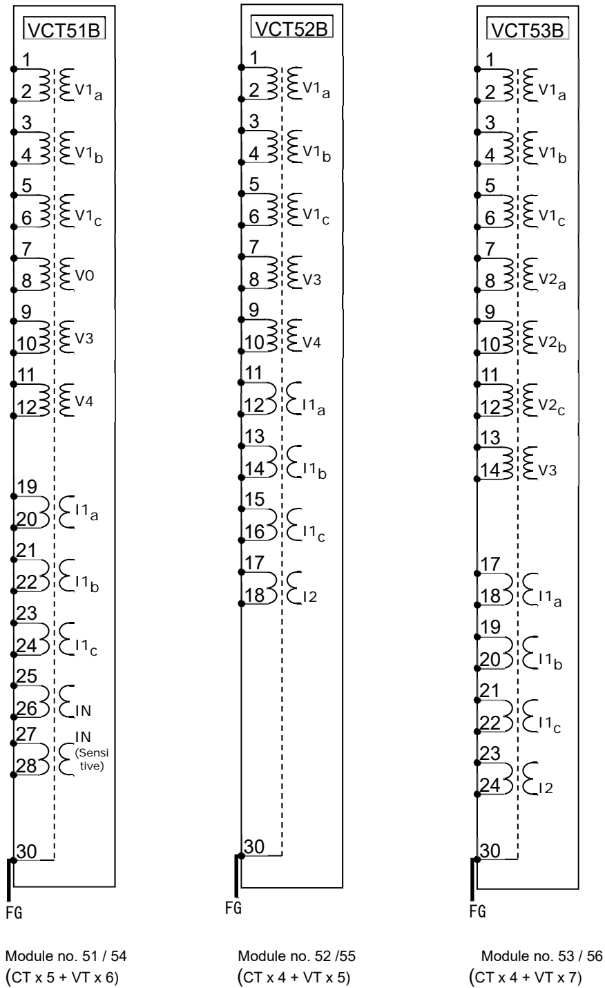
Figure 14 – CT/VT module
