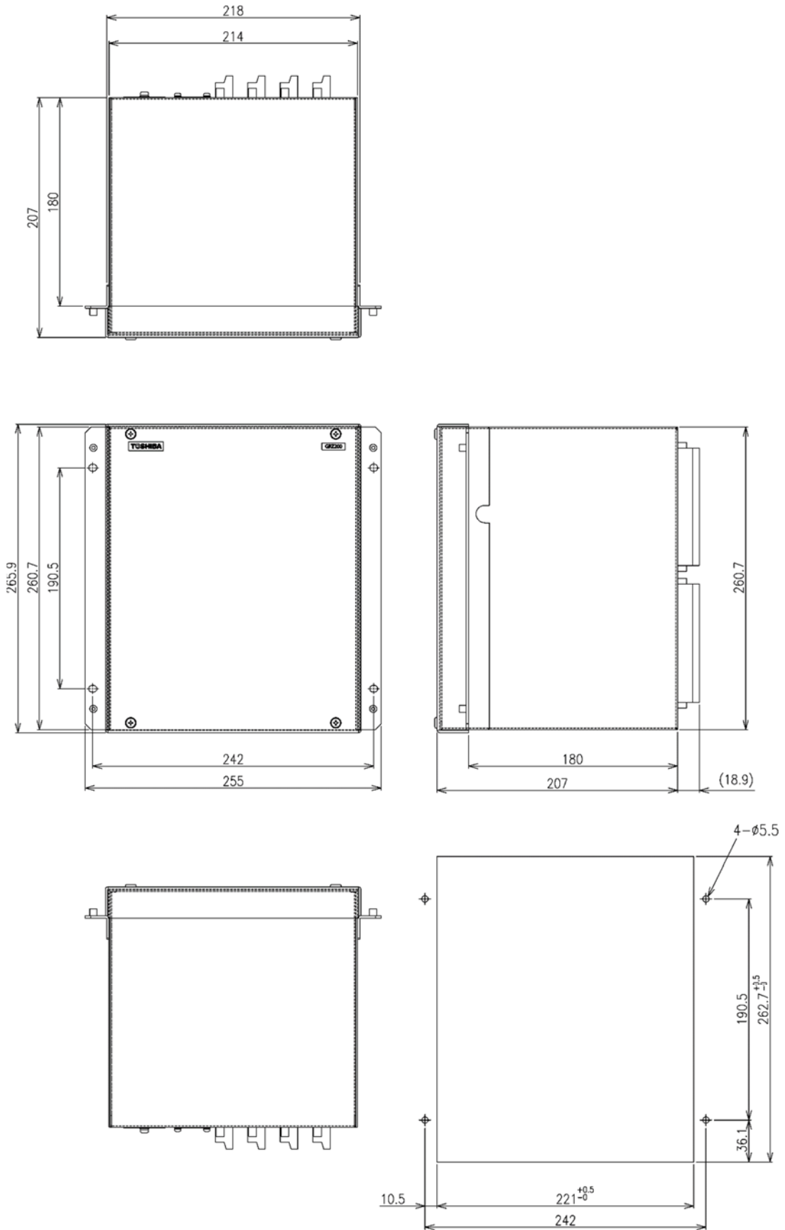
Figure 16 – Dimension and Panel Cut-out – 1/2 x 19” case size
