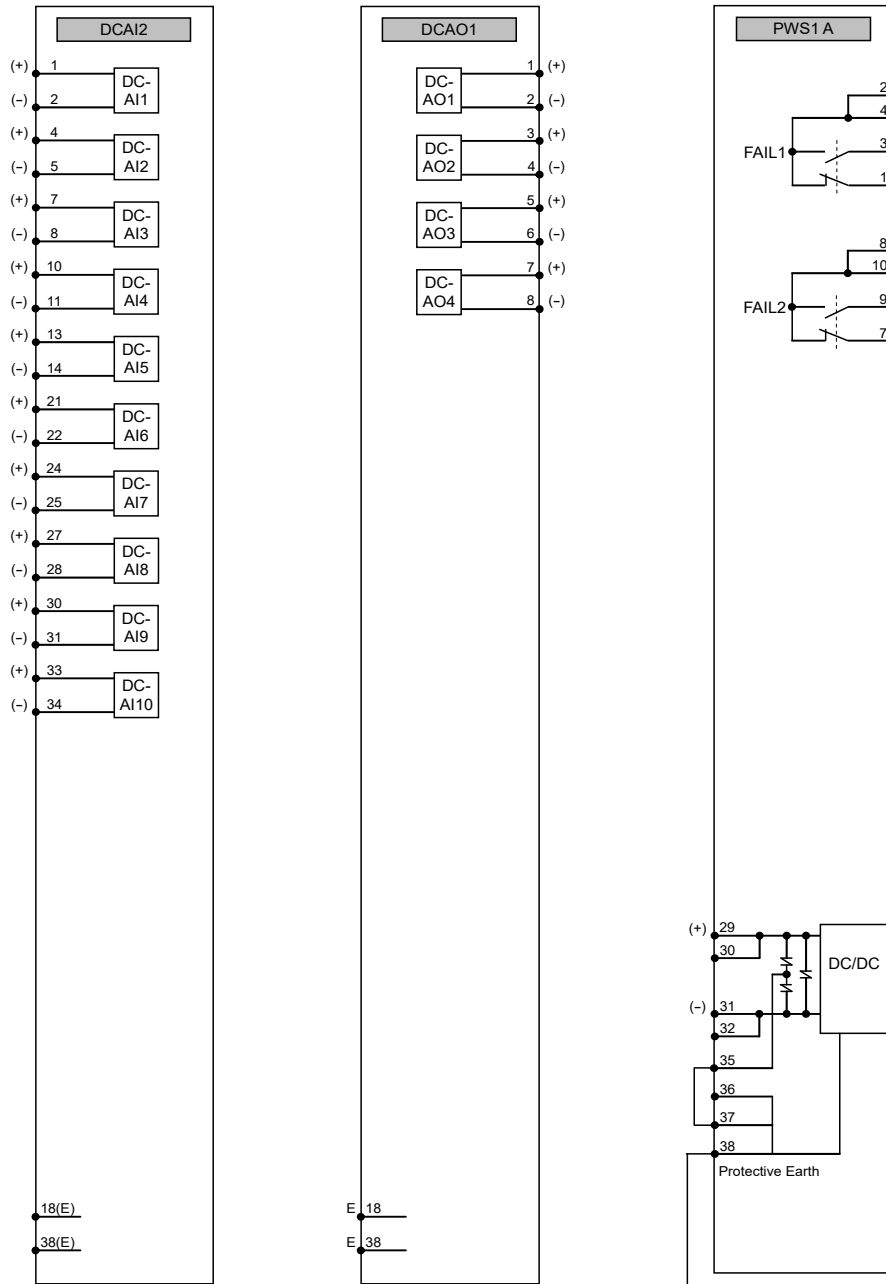
Figure 13 – DC-analogue input and output module and DC/DC module
